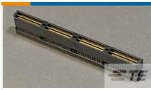
TE Part # 3-1658439-4 MSB0.80PL14ASY112DP,GP,30,VCTY
